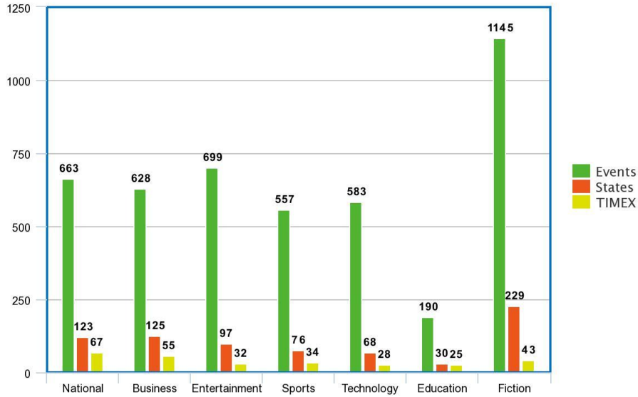
Figure 2: Domain Wise Distribution for Event, State and TIMEX tags
